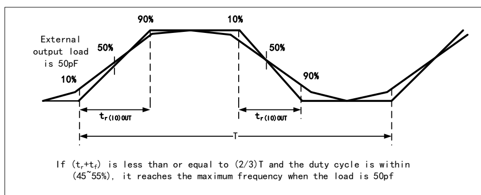
Figure 13 I/O AC Characteristics Definition
