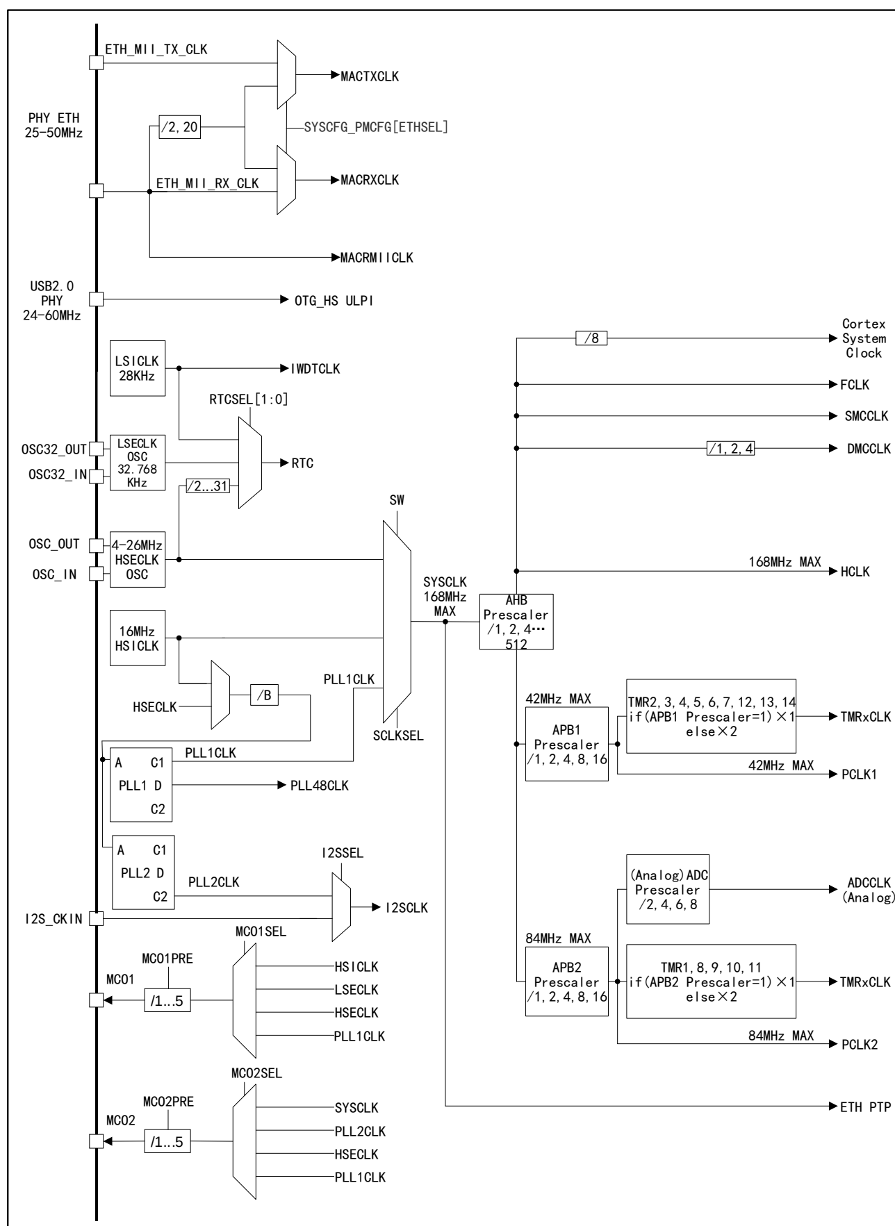
Figure 8 APM32F405xG 407xExG Clock Tree
