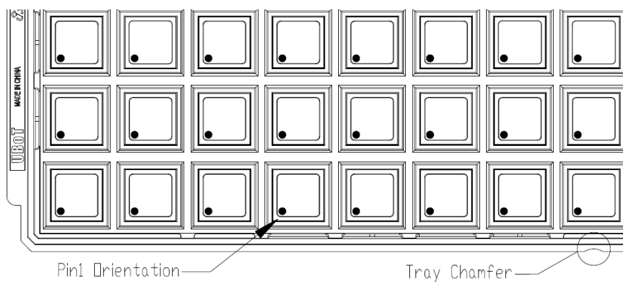
Figure 32 Tray Packaging Diagram
